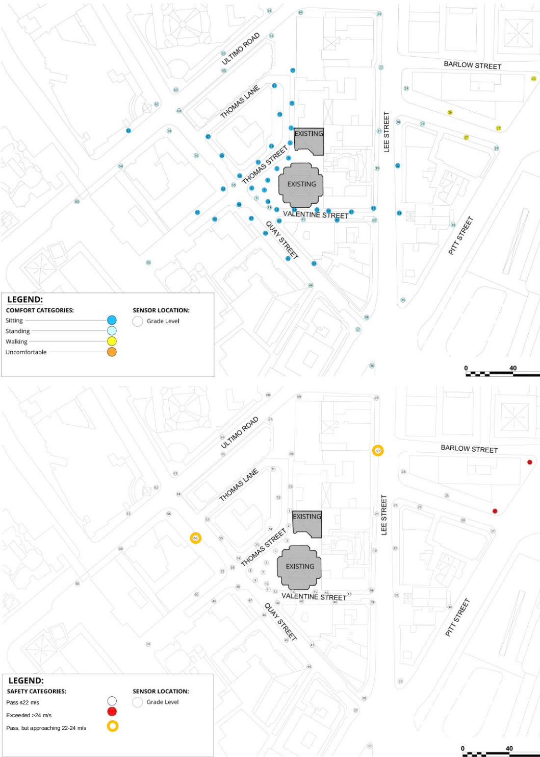
Figure 5: Existing configuration comfort (T) and safety(B) wind rating
