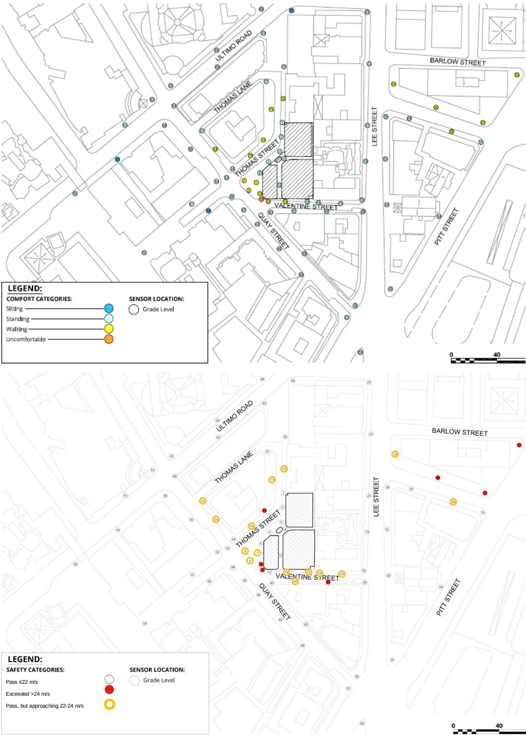
Figure 7: Proposed configuration comfort (T) and safety(B) wind rating
